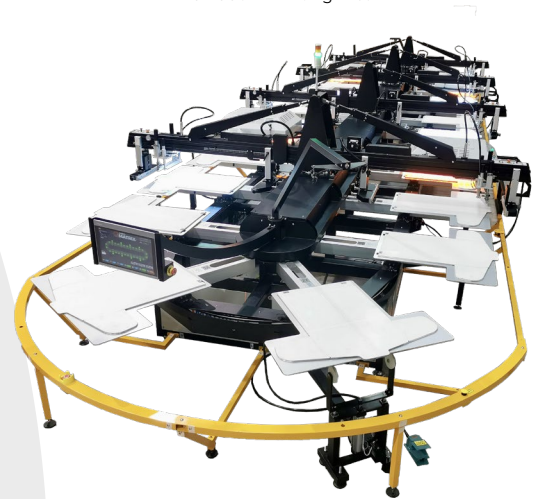
All Over Oval Printing Press Prints on every part of the shirt.
